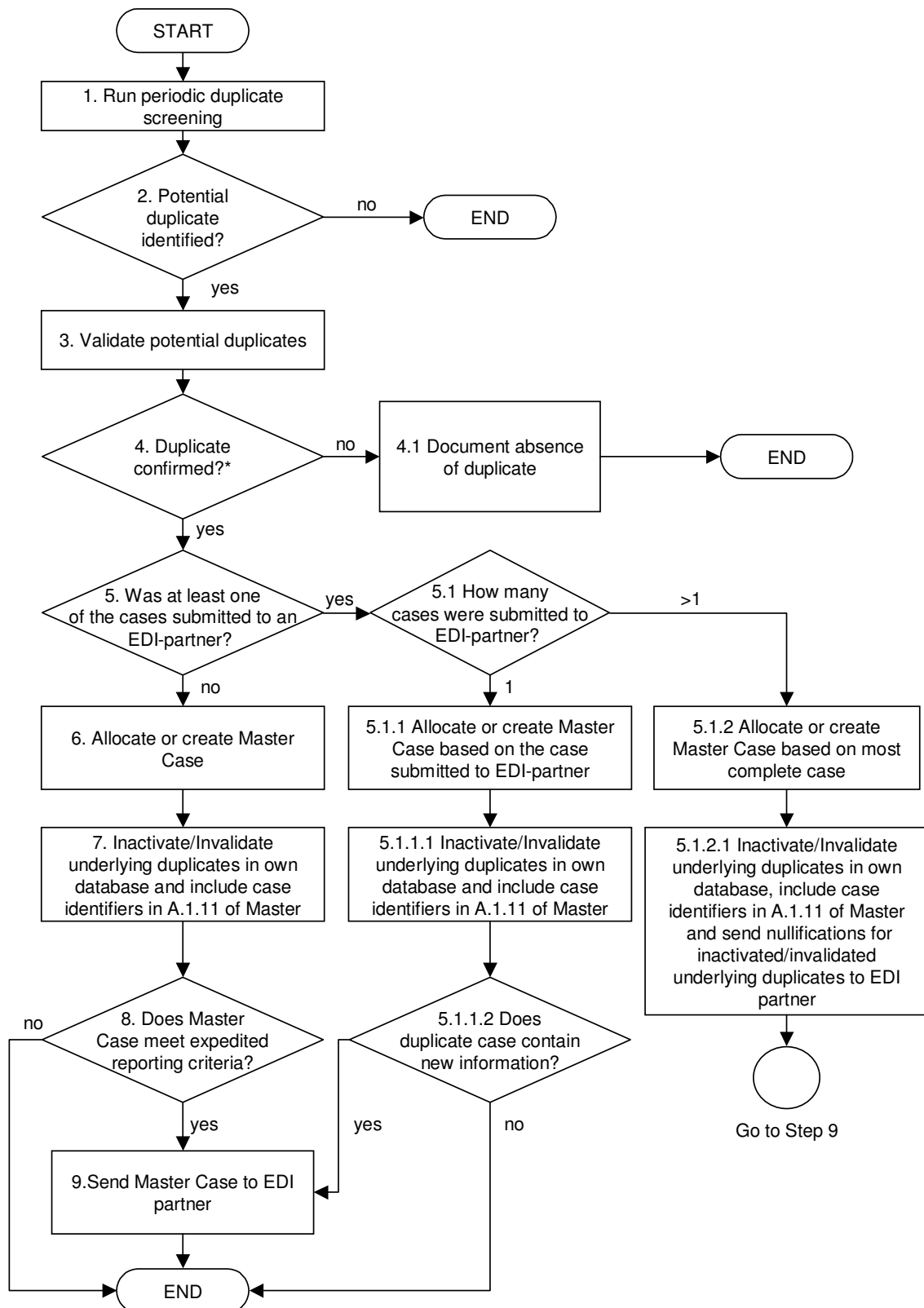
Flowchart 1 Process of allocating or creating a 'master case' of duplicates existing in a database
